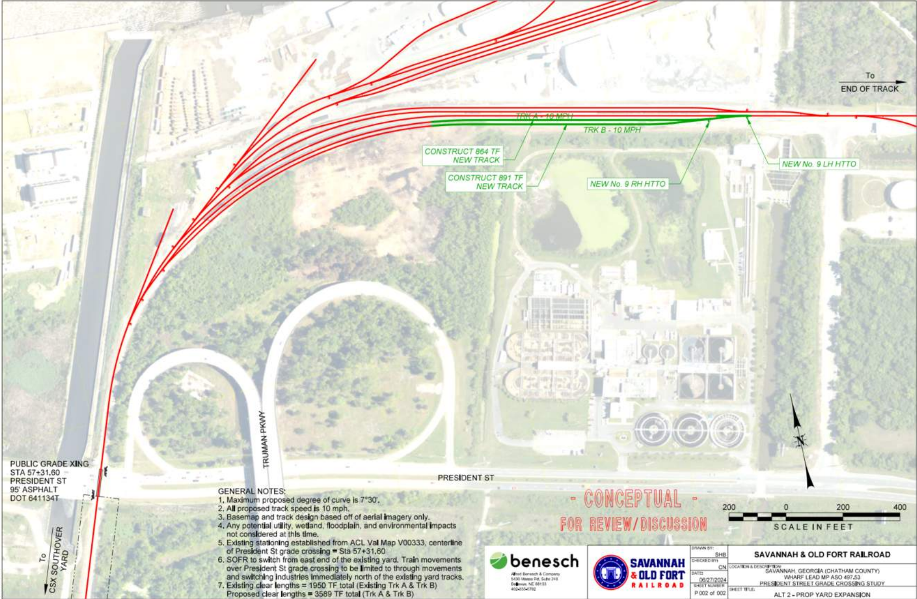
Figure 28: Alternative 8: Extend Storage Tracks Within Wharf Rail Yard
